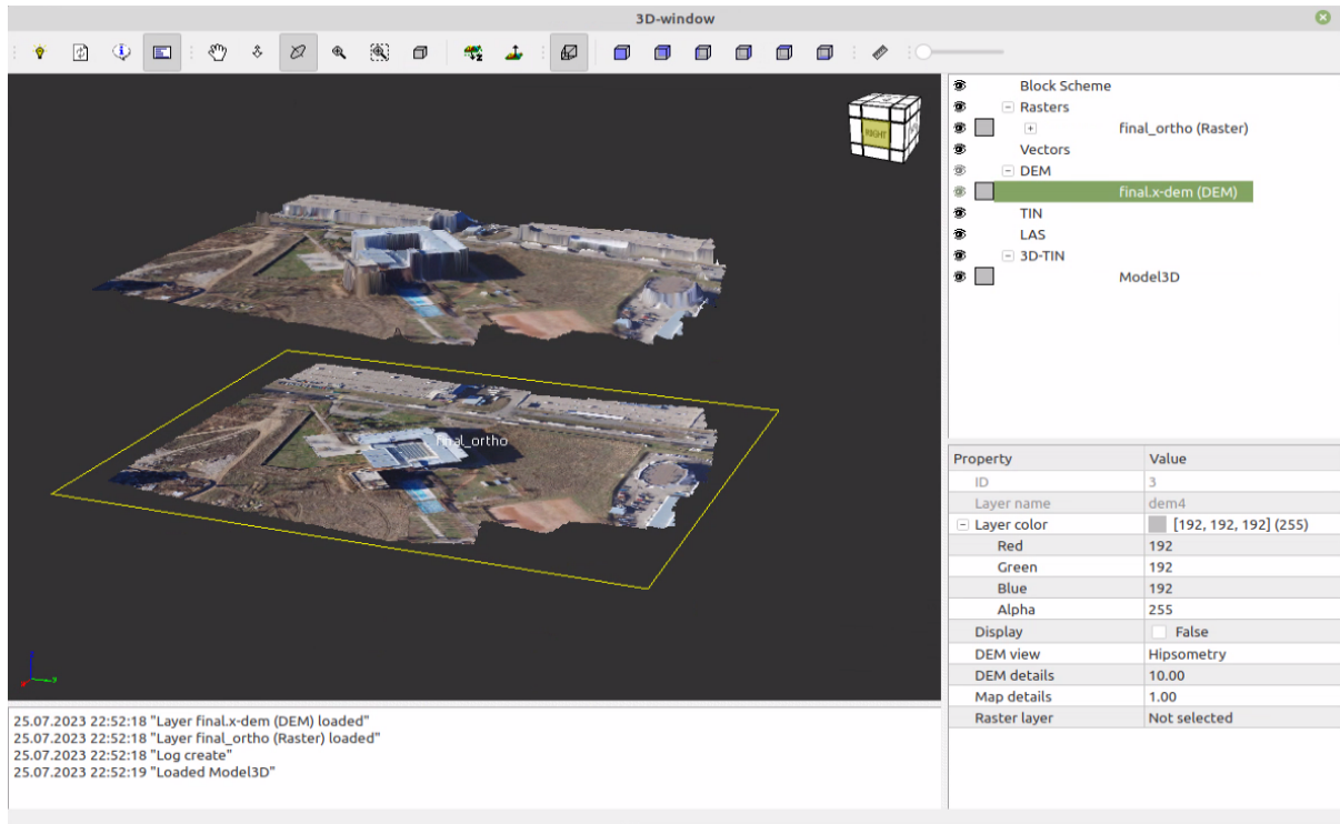
Fig. 27. 3D-window
