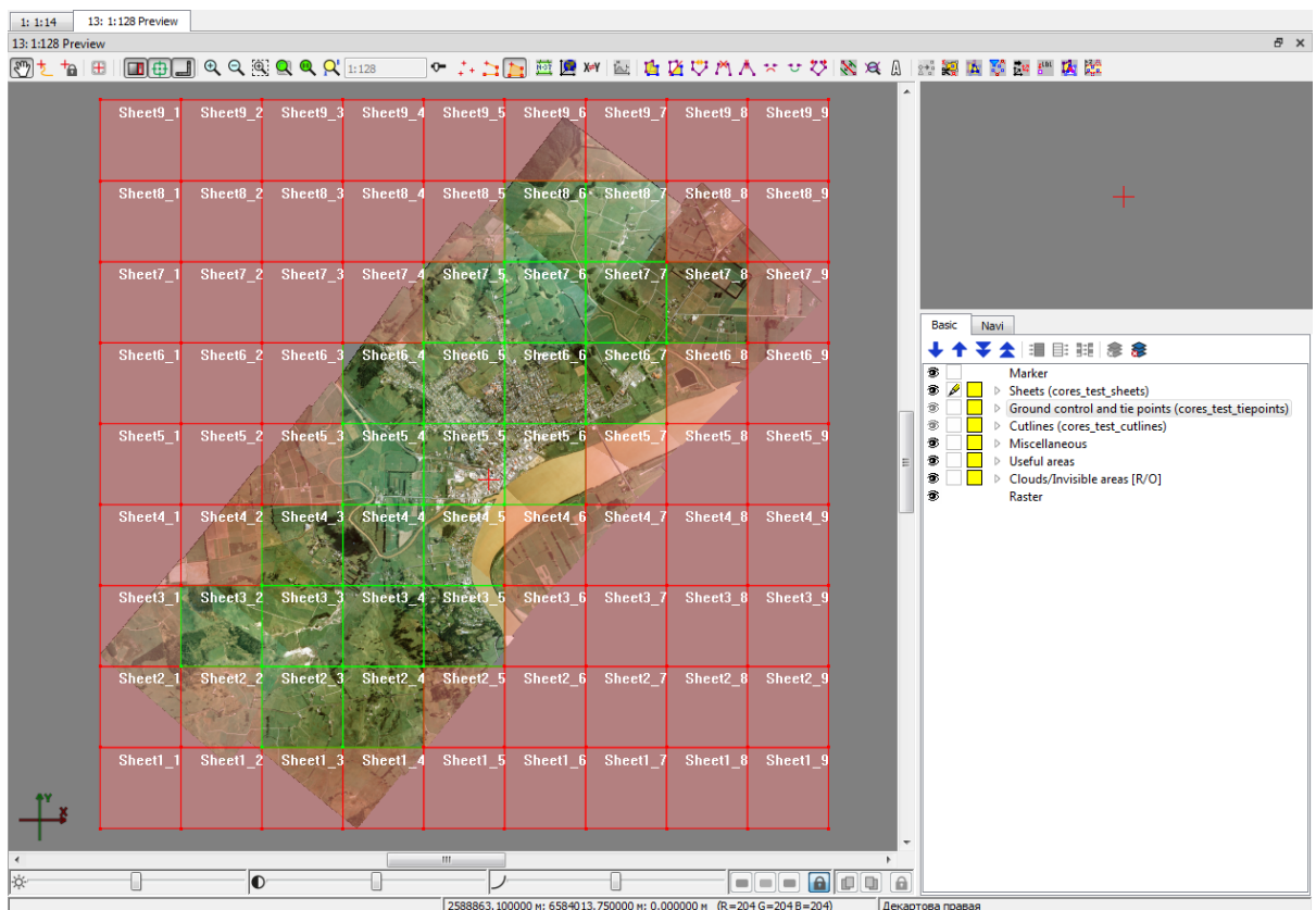
Fig. 48. Sequential splitting
