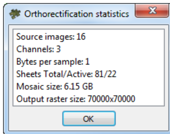
Fig. 4. Project information
