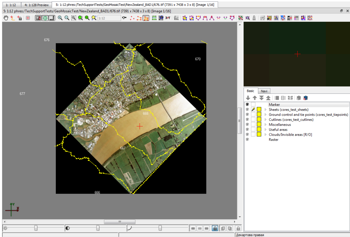
Fig. 10. Project image
