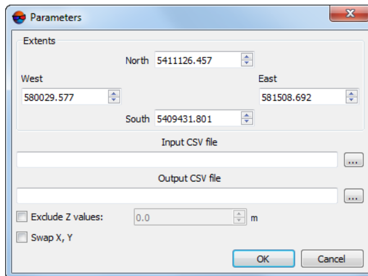
Fig. 191. Parameters of CSV file cutting by rectangle boundaries
