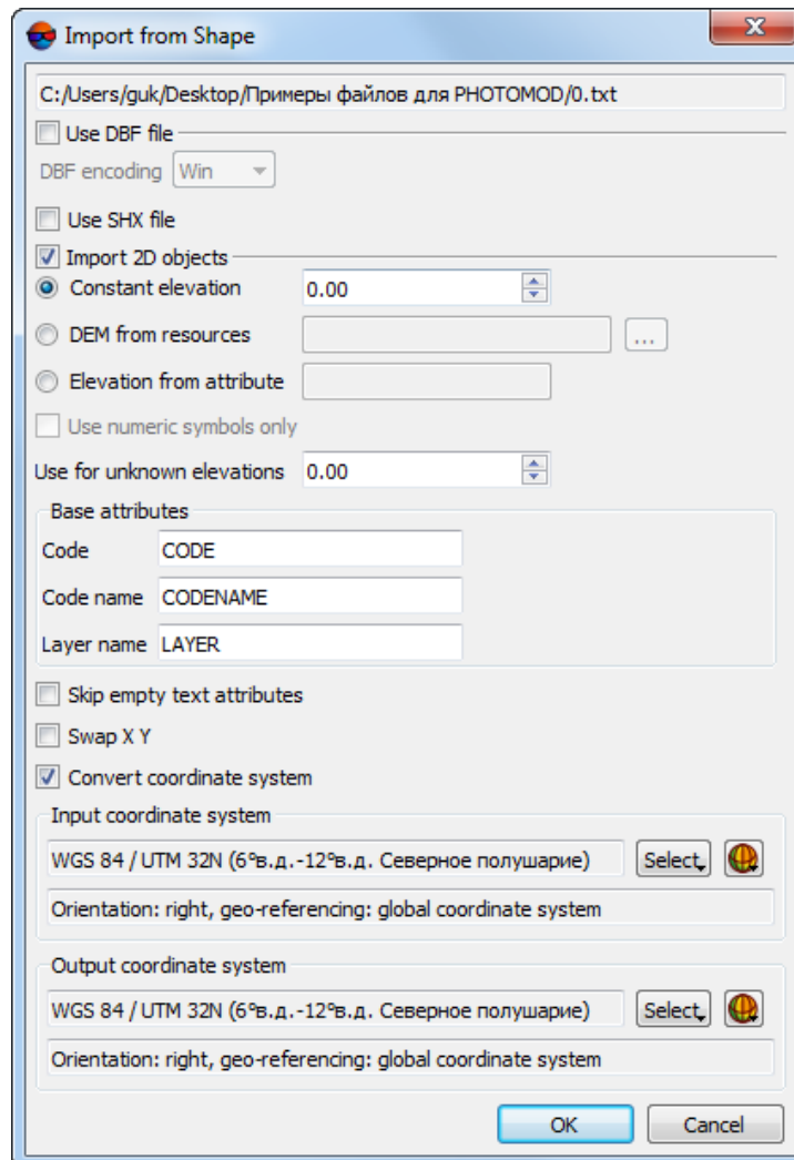
Fig. 230. Import from SHP format
