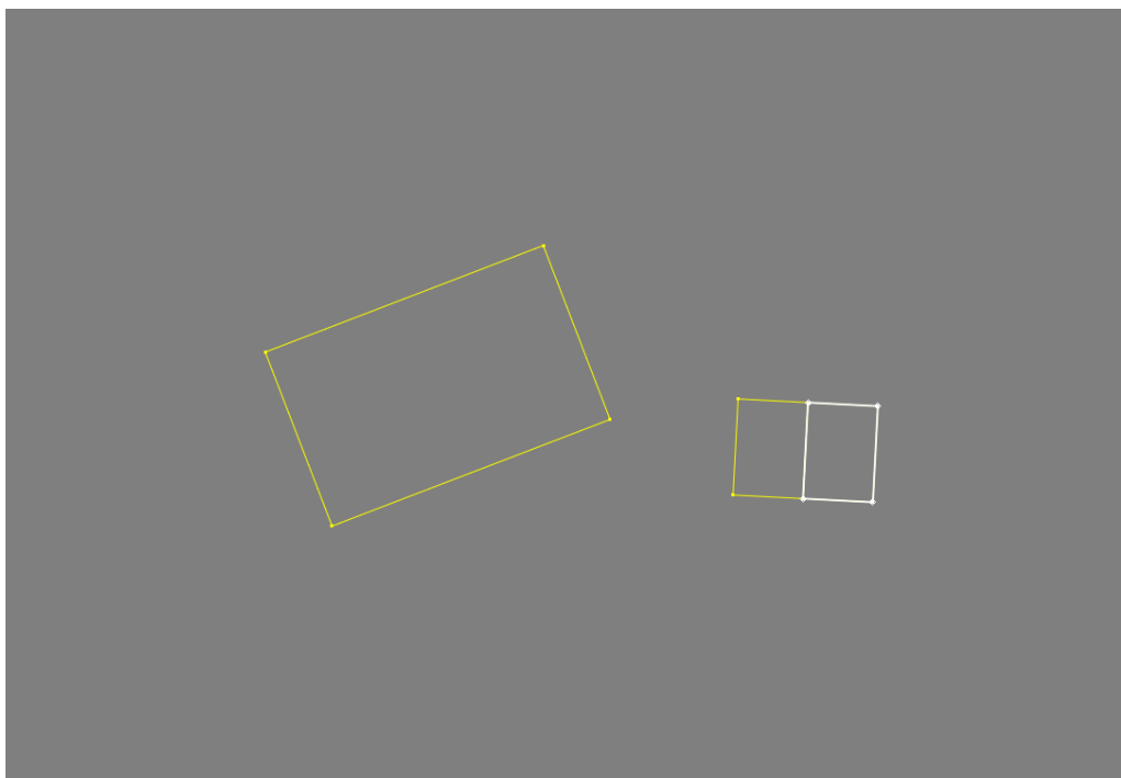
Fig. 165. A gable roof consisting of two vector objects (the right pitch is selected).
