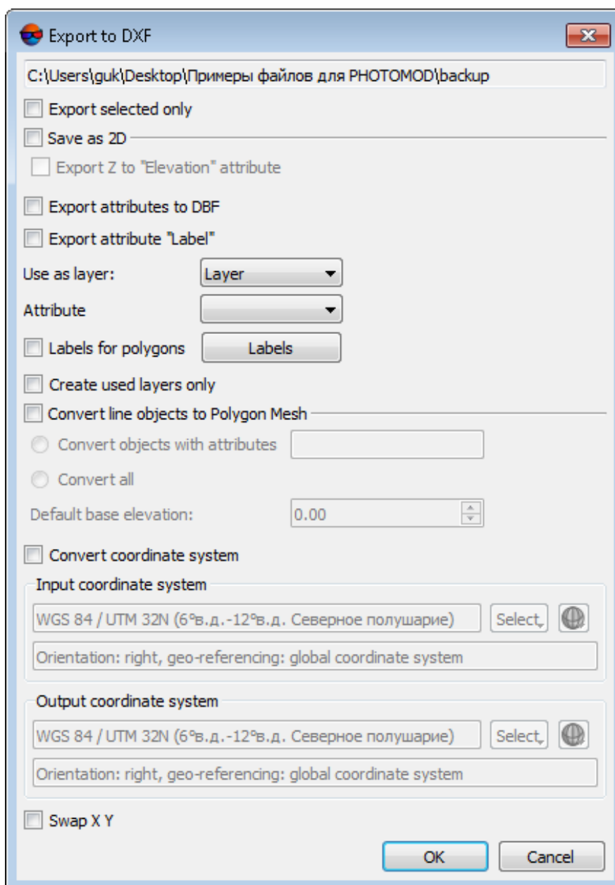
Fig. 244. Batch export to DXF format
