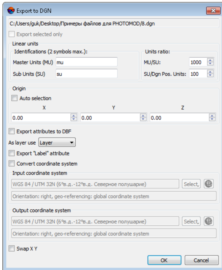
Fig. 238. Export to DGN format
