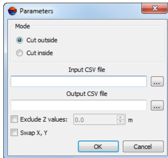
Fig. 192. Parameters of CSV file cutting by selected polygons
