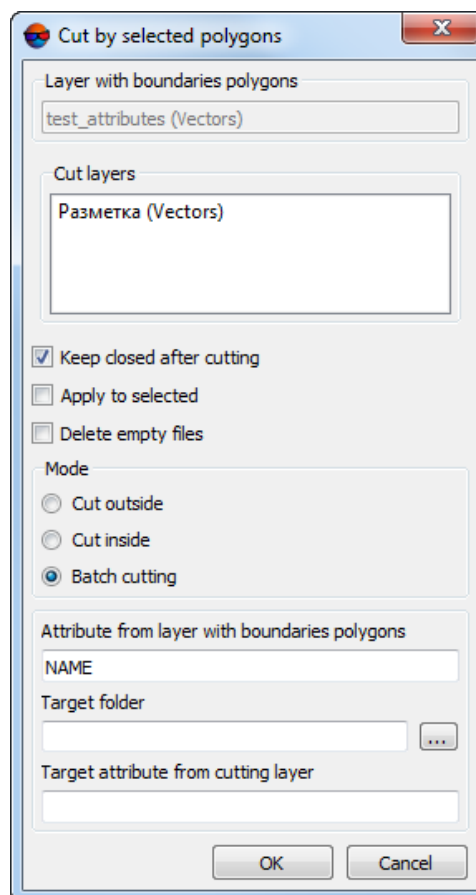
Fig. 152. Parameters of batch cutting by polygons
