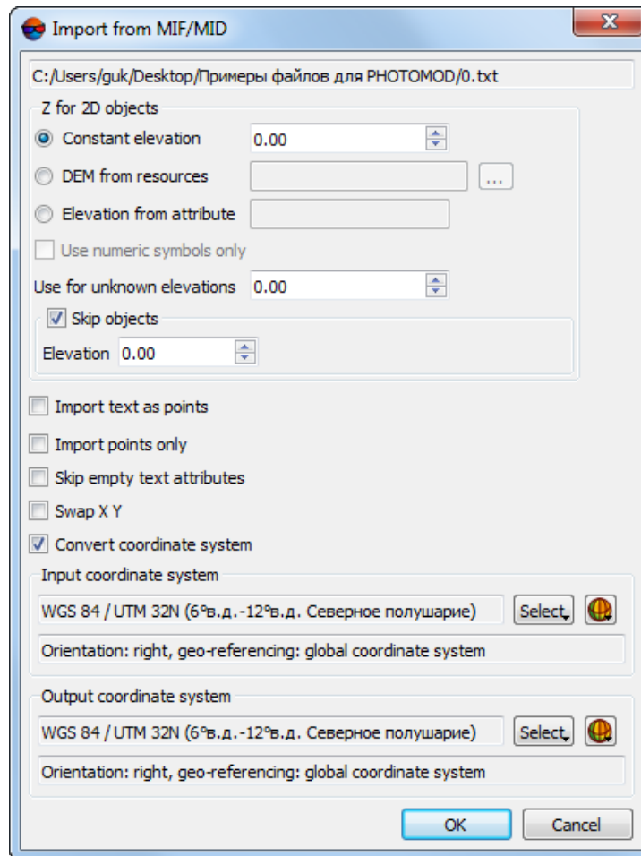
Fig. 229. Import from MIF/MID format
