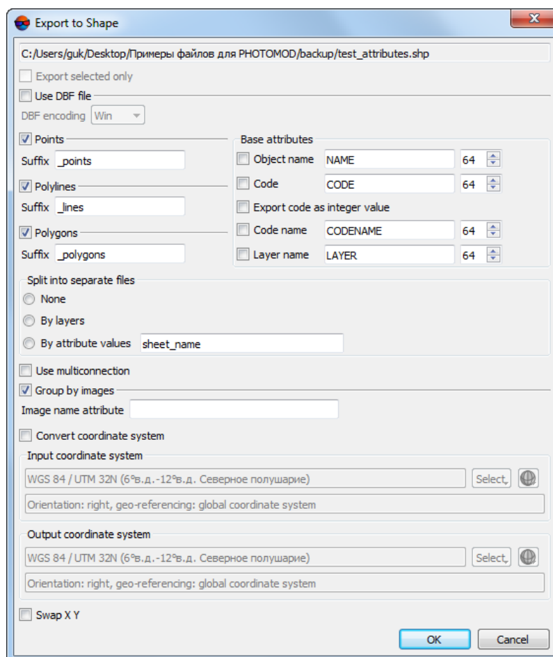
Fig. 251. Export to SHP format
