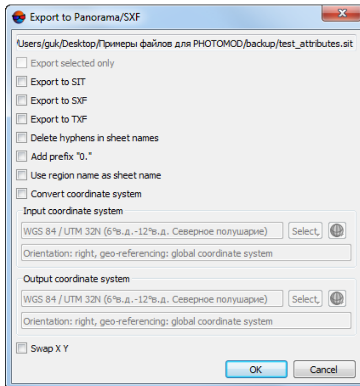
Fig. 252. Export to Panorama / SXF
