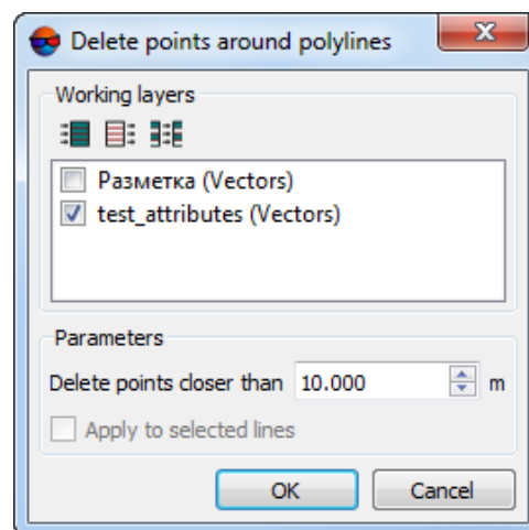
Fig. 187. Parameters of deleting points around linear objects
