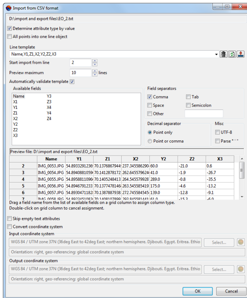
Fig. 220. Import from CSV
