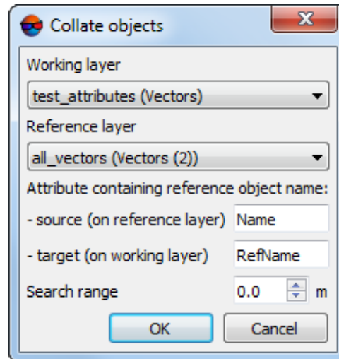
Fig. 108. Parameters of objects collation
