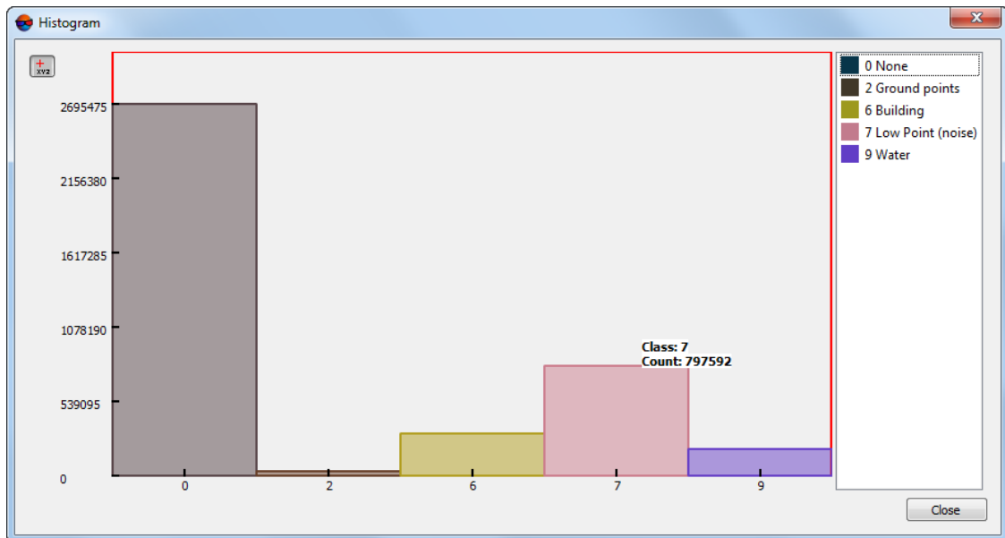
Fig. 33. The Histogram window (according to LIDAR points classification)
