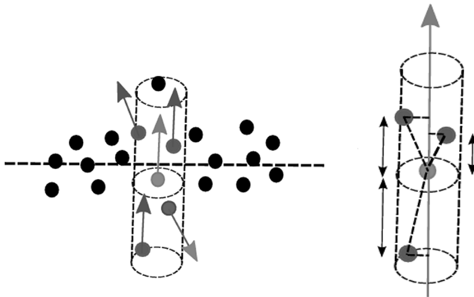
Fig. 39. Filter working principle
